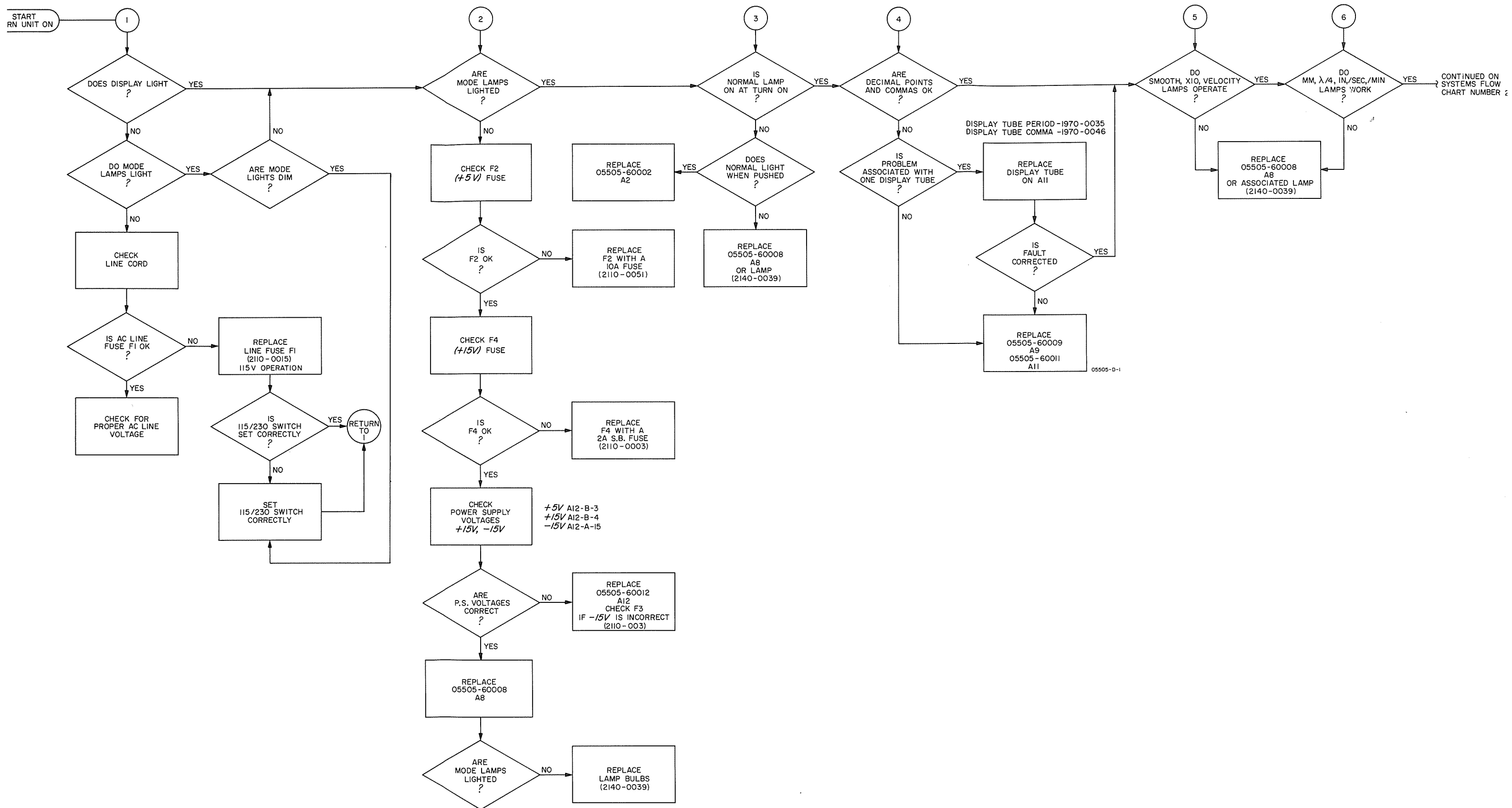
Figure 5-23 TROUBLESHOOTING TREE (Sheet 1 of 4)
